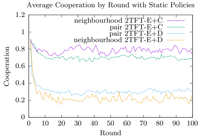
Fig. 3. Results from the average of 100 100 round tournaments with four different sets of agents. All the sets have two Tit-for-Tat (TFT) agents with 10% exploration. Two have a third agent that always defects, and two have one that always cooperates. The other variable is voting (pairwise or neighbourhood).
