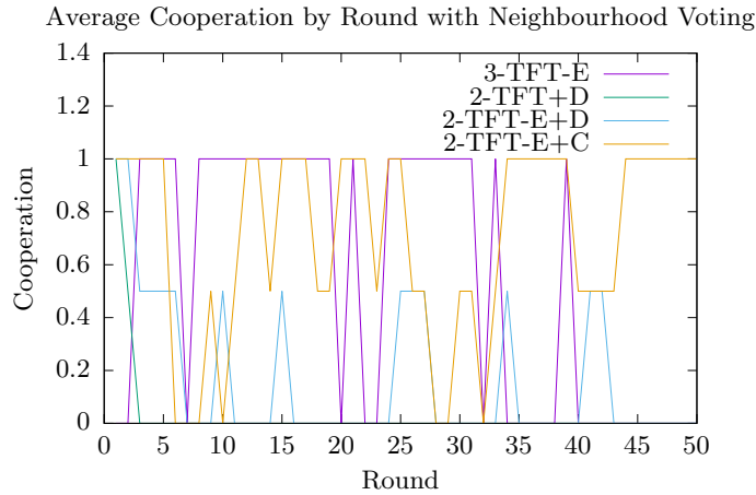
Fig. 2. Results from four 50 round tournaments with static agents with neighbourhood voting. 3-TFT-E refers to 3 Tit-for-Tat agents with 10% exploration that start cooperating. 2-TFT+D refers to two TFT agents with an agent that always defects; this quickly descends to no cooperation. 2-TFT-E+D refers to two TFT agents with exploration and an always defect agent; this system has some cooperation but mostly defects, but more than with pairwise voting. 2-TFT-E+C refers to two TFT exploration agents and an agent that always cooperates; this cooperates about 75% of the time.
